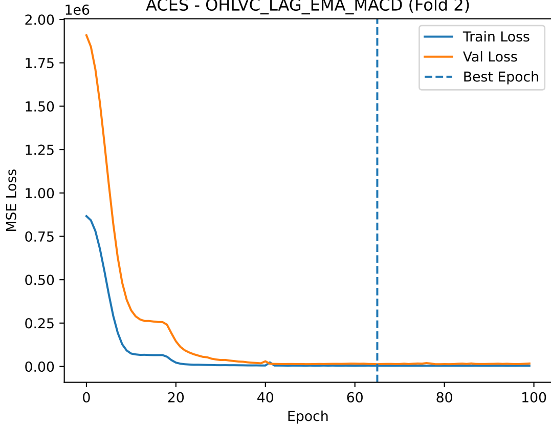
ACES - OHLVC_LAG_EMA_MACD (Fold 2)
